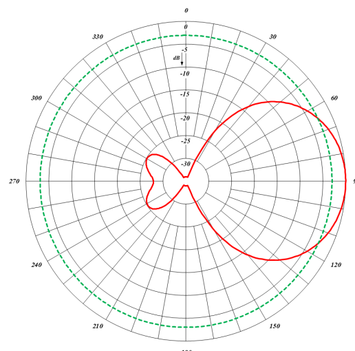
Vertical pattern 680-1690 Vertical Polarization
