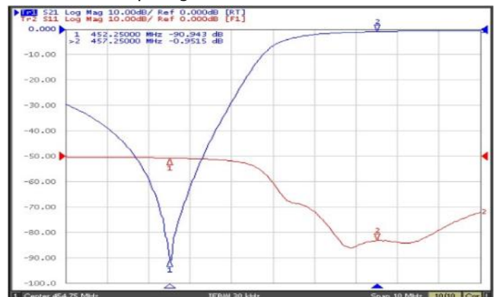
506-90 Typical Response Curves at 5 MHz Spacing
