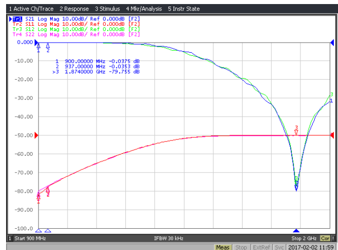
Typical 900MHz Curve:
