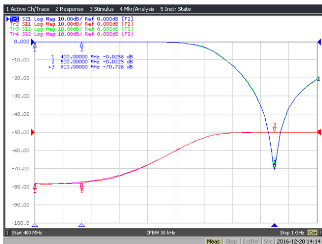
Typical UHF Curve:
