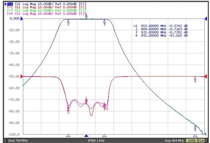
800MHz Pass: 809-821MHz (12MHz)
