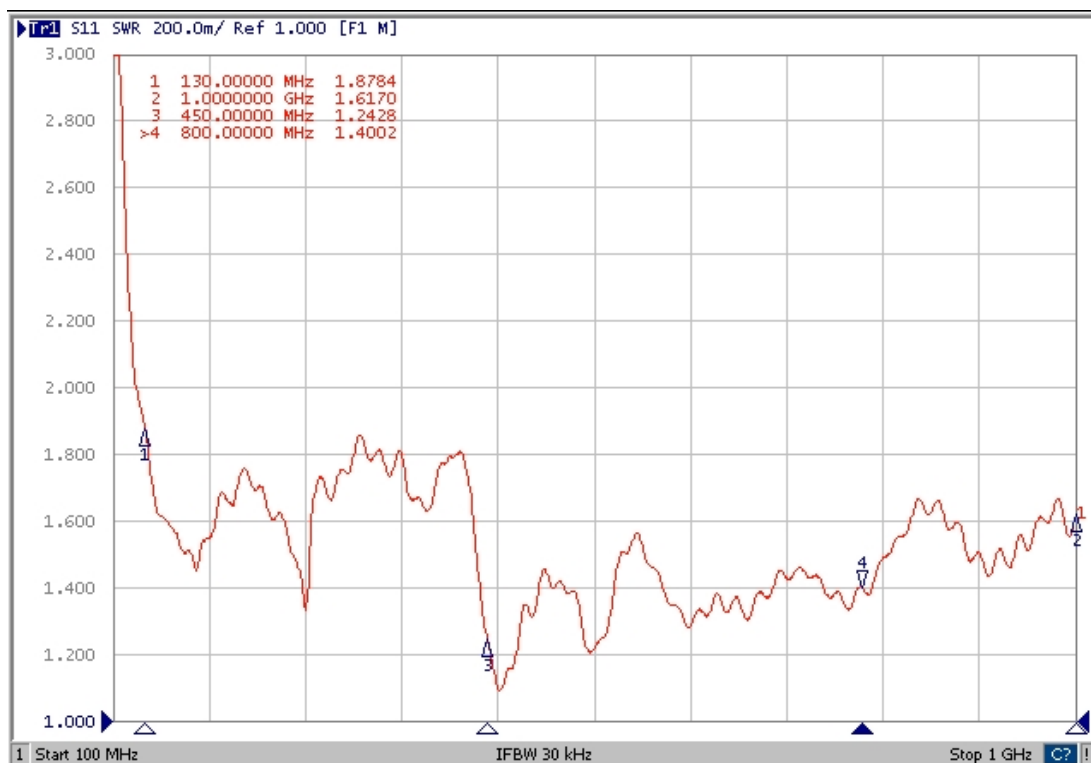
VSWR Curve Representative of all models
