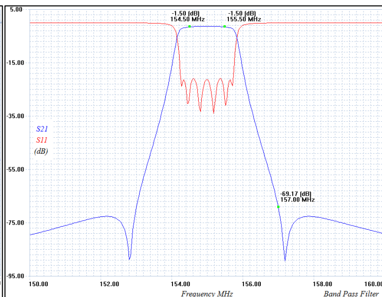
59-13-46 Electrical Response
