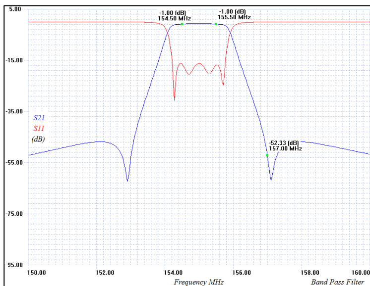
59-13-44 Electrical Response
