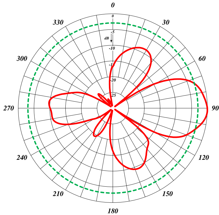
Radiation pattern Vertical
