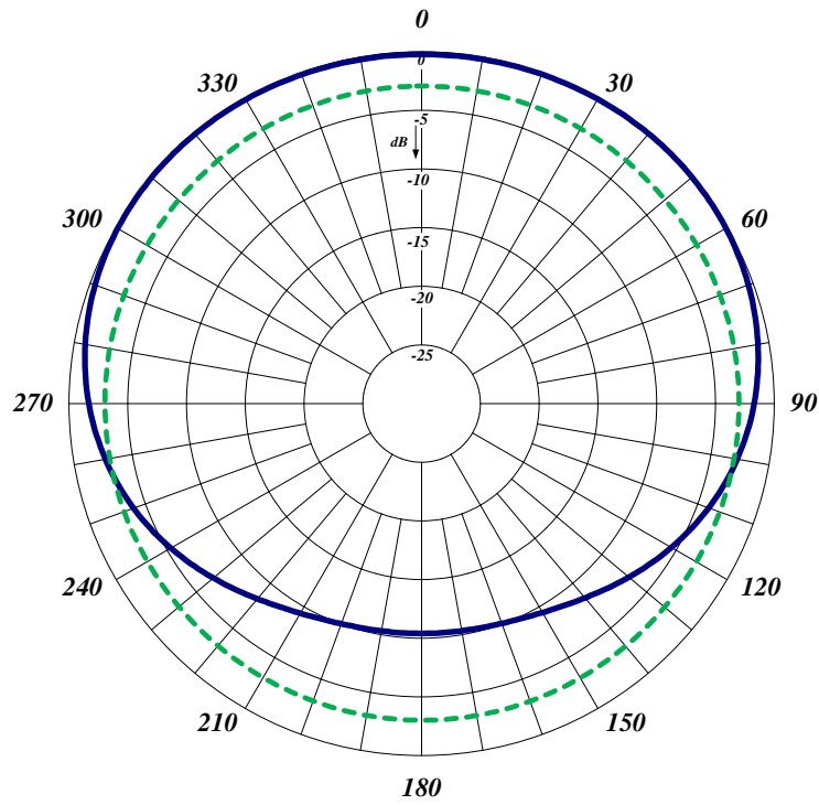
Radiation pattern Horizontal
