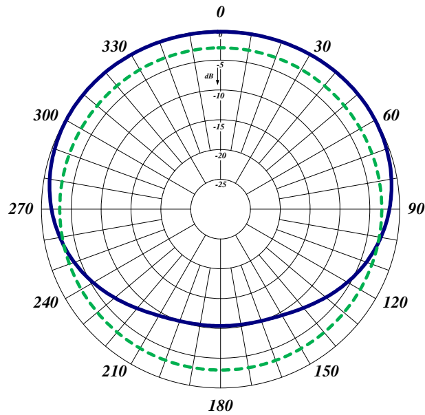
Quater-wave Spacing
