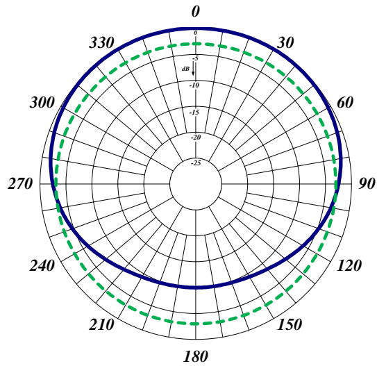
Quater-wave Spacing
