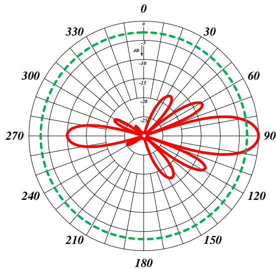
Quater-wave Spacing Vertical
