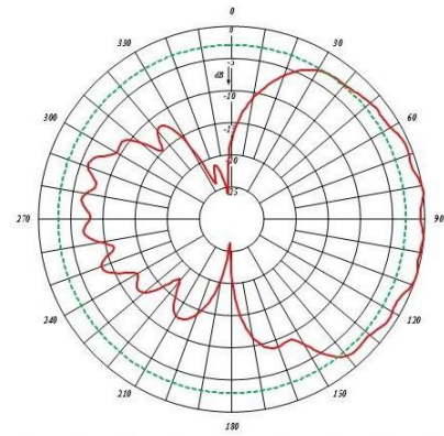
UHF: vertical pattern
