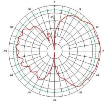
UHF: vertical pattern
