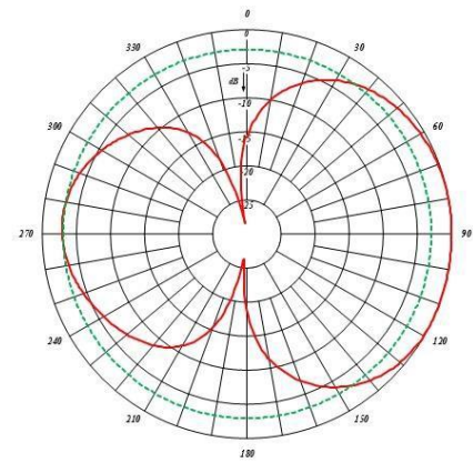
VHF: vertical pattern
